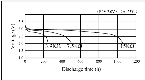
Discharge characteristics
