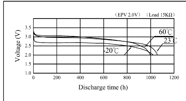
Temperature characteristics
