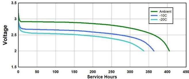
Cold Temperature Performance 5 kOhm Continuous to 2.0V
